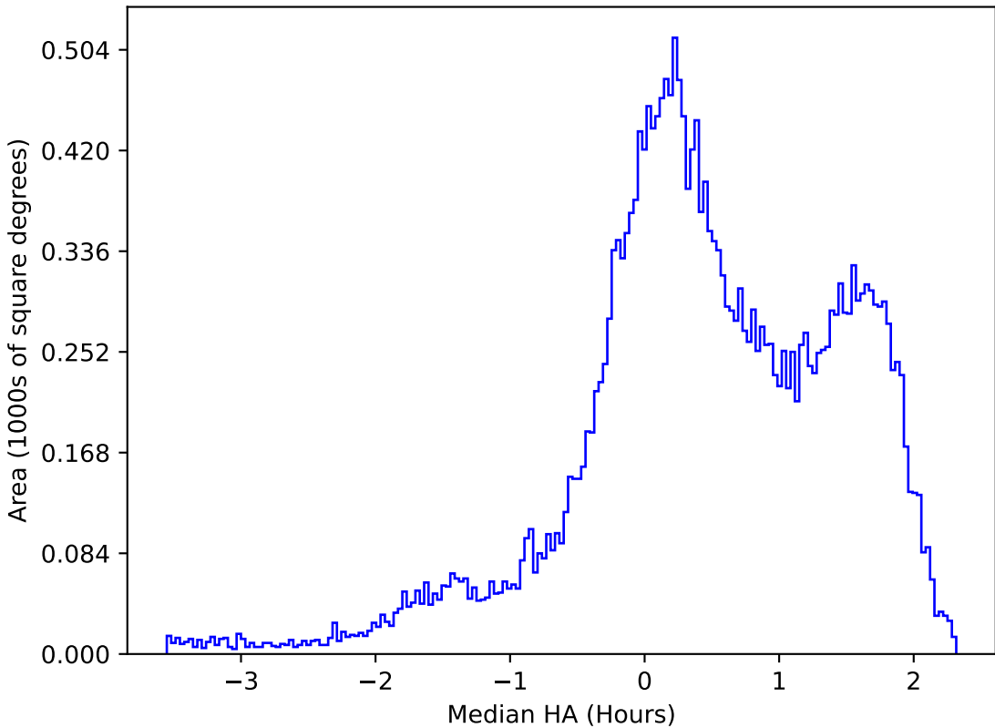
too_elab_r64_d2_giz_v3.4_10yrs All sky g band: Median HA
