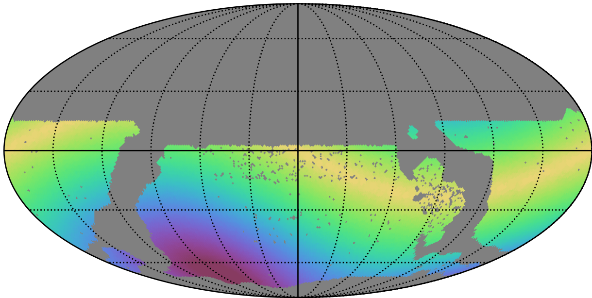
too_elab_r64_d2_giz_v3.4_10yrs WFD z band: Max solarElong
