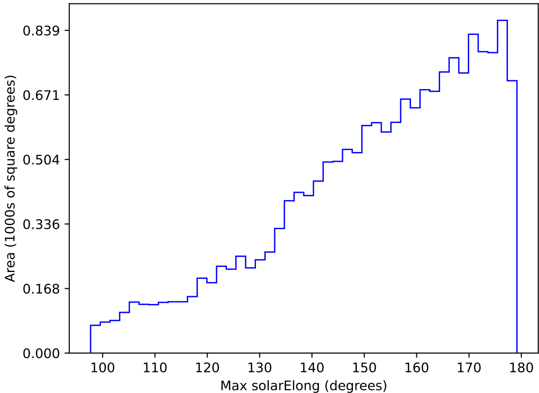
too_elab_r64_d2_giz_v3.4_10yrs WFD u band: Max solarElong
