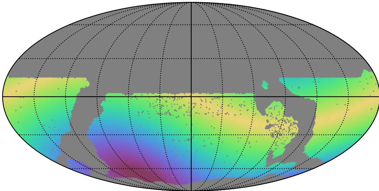
too_elab_r64_d2_giz_v3.4_10yrs WFD r band: Max solarElong
