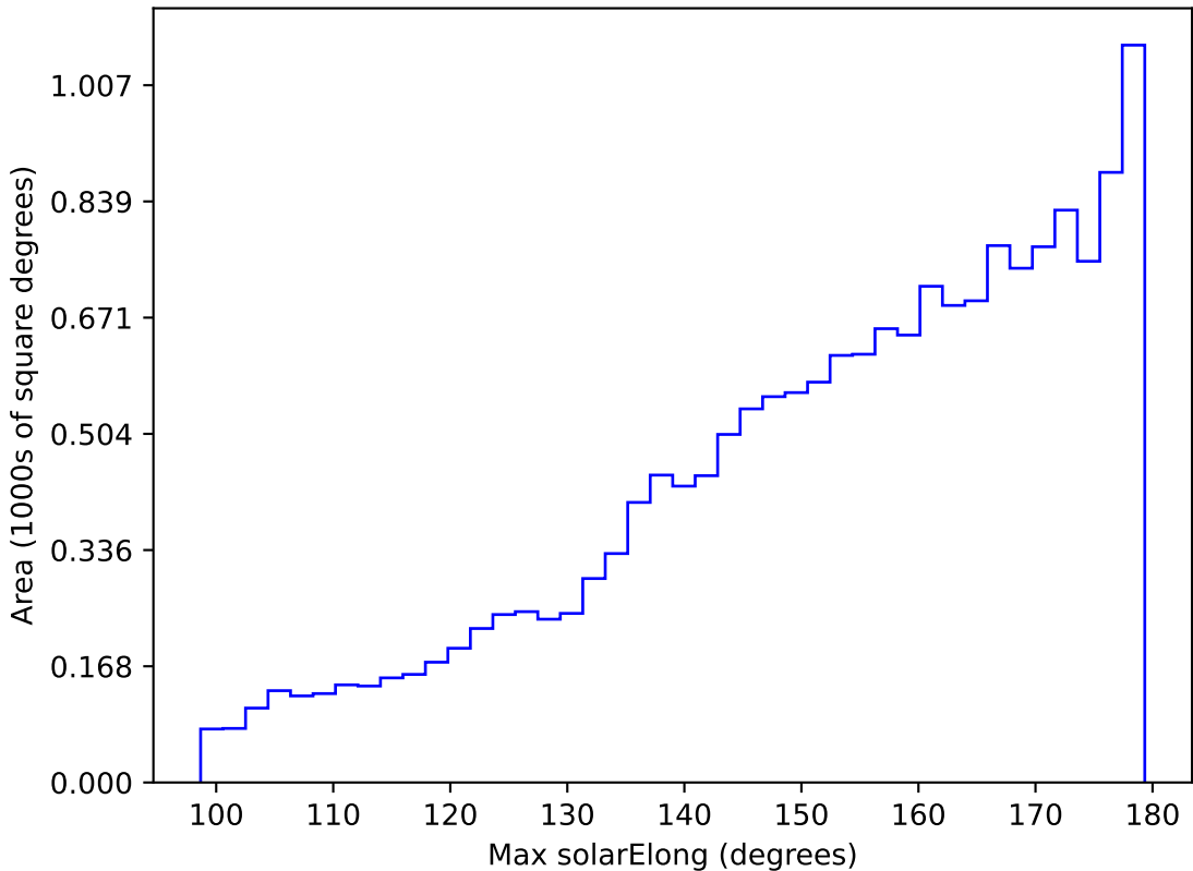
too_elab_r64_d2_giz_v3.4_10yrs WFD r band: Max solarElong
