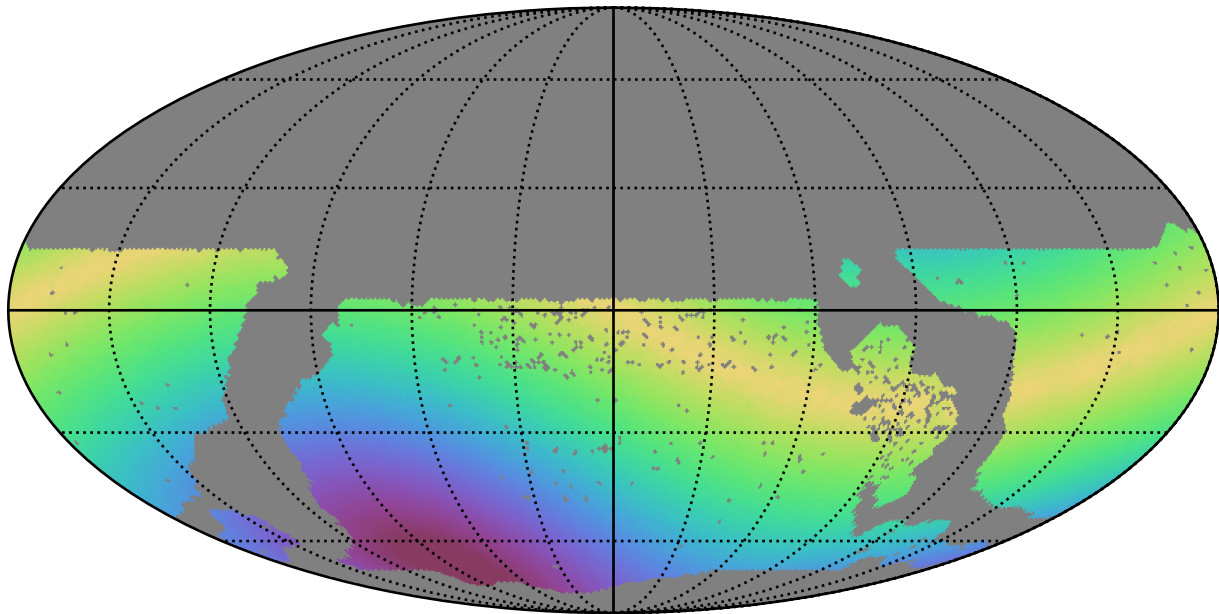
too_elab_r64_d2_giz_v3.4_10yrs WFD i band: Max solarElong
