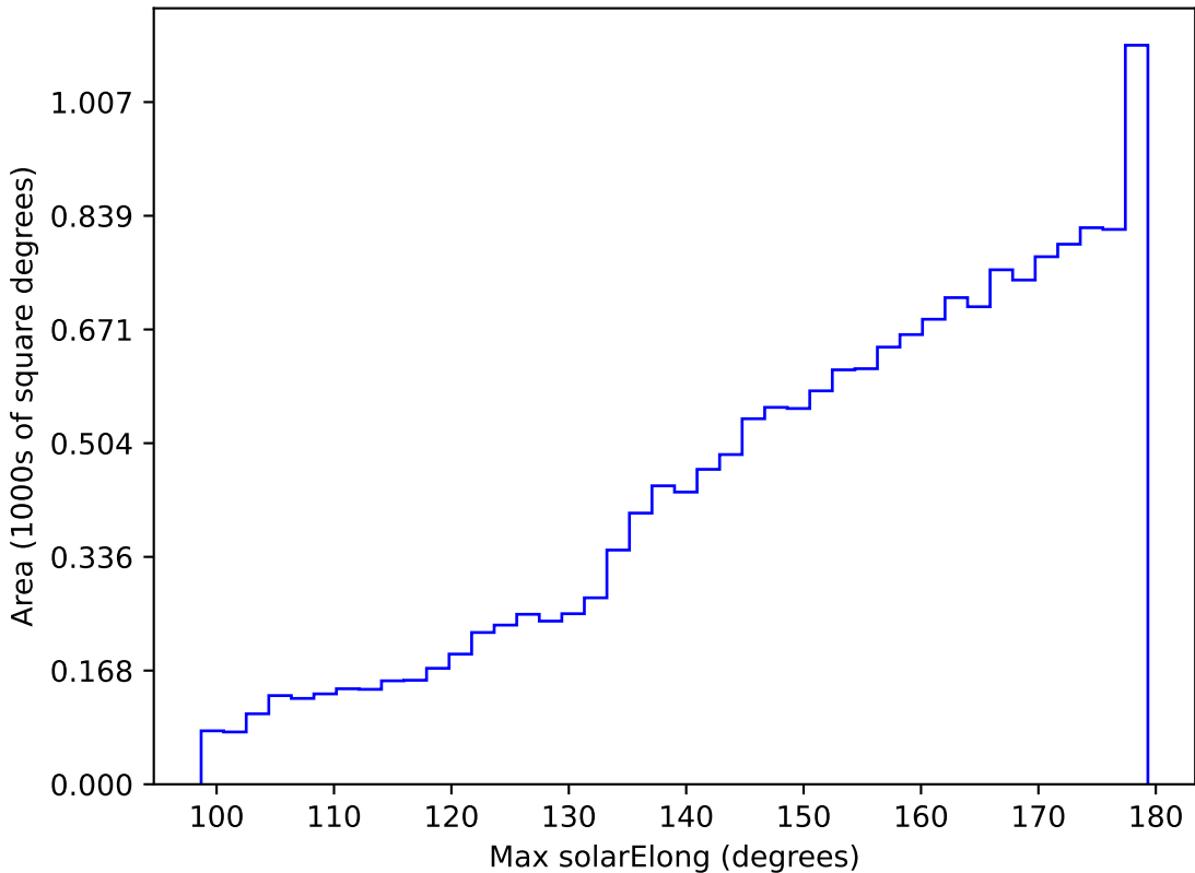
too_elab_r64_d2_giz_v3.4_10yrs WFD i band: Max solarElong
