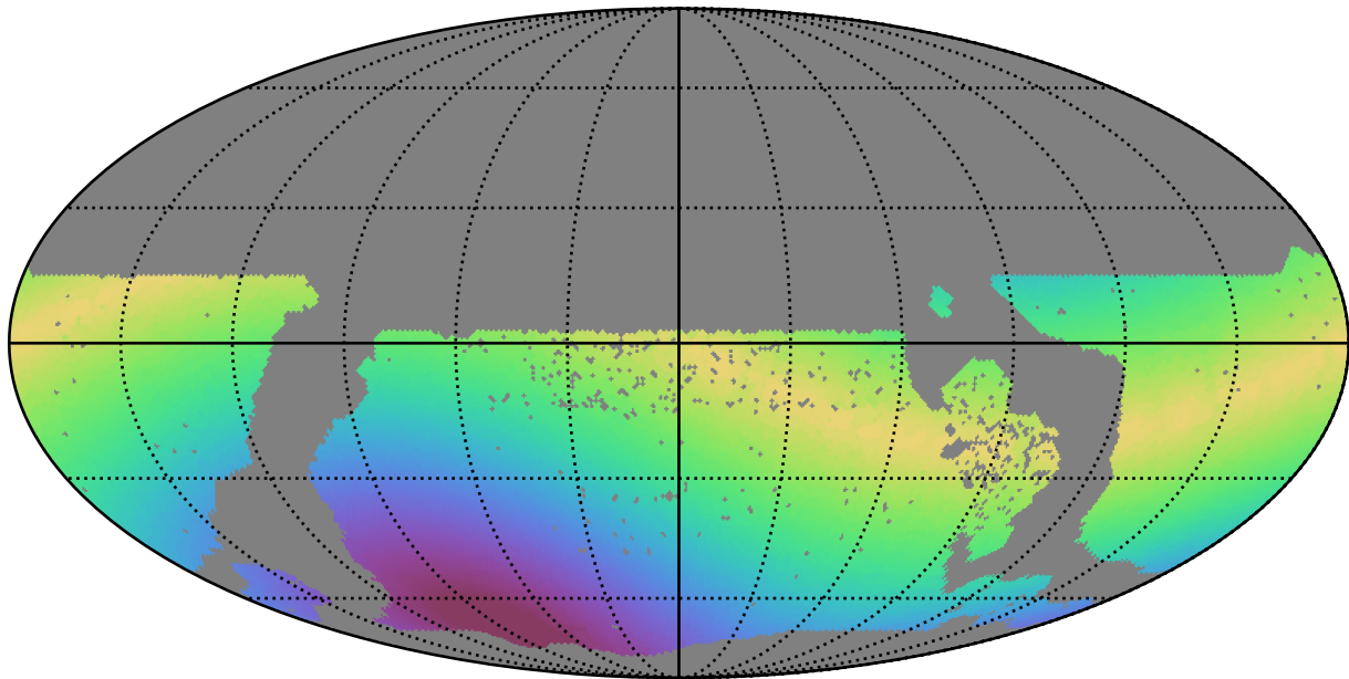
too_elab_r64_d2_giz_v3.4_10yrs WFD g band: Max solarElong
