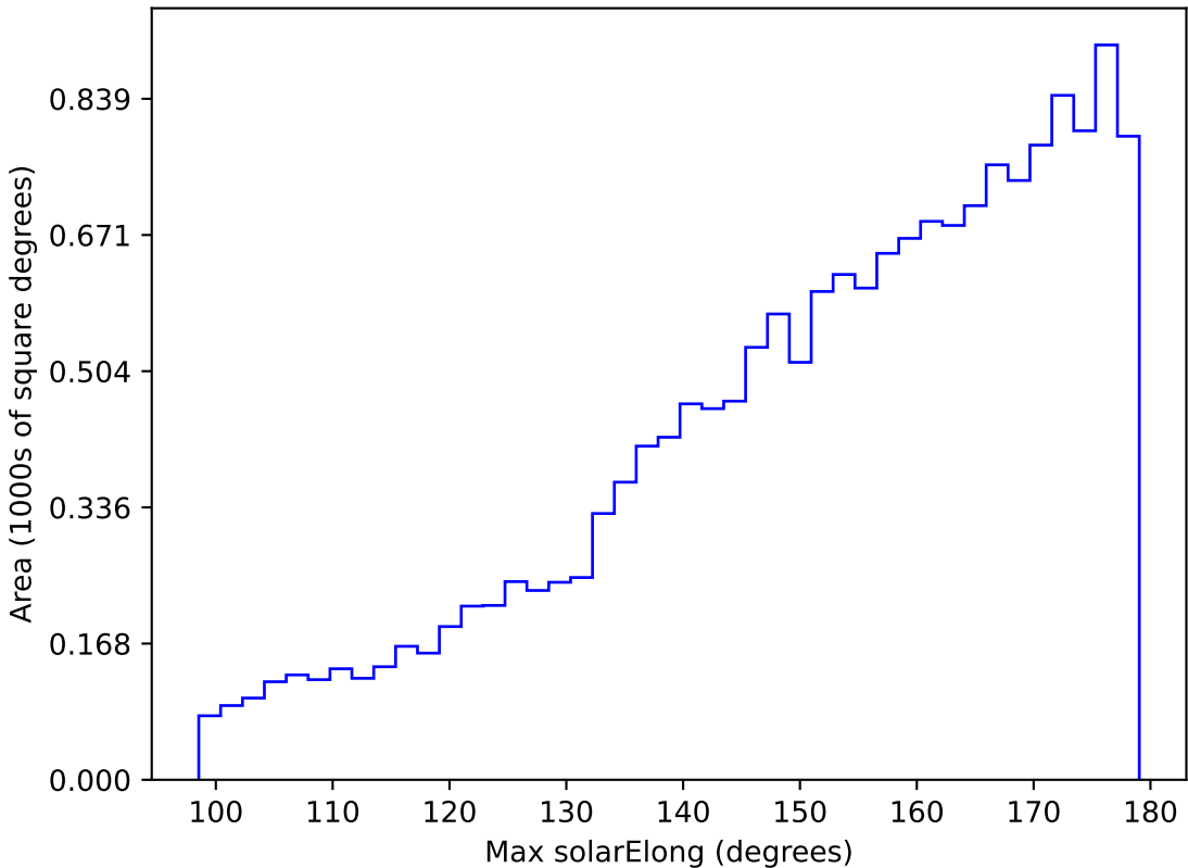
too_elab_r64_d2_giz_v3.4_10yrs WFD g band: Max solarElong
