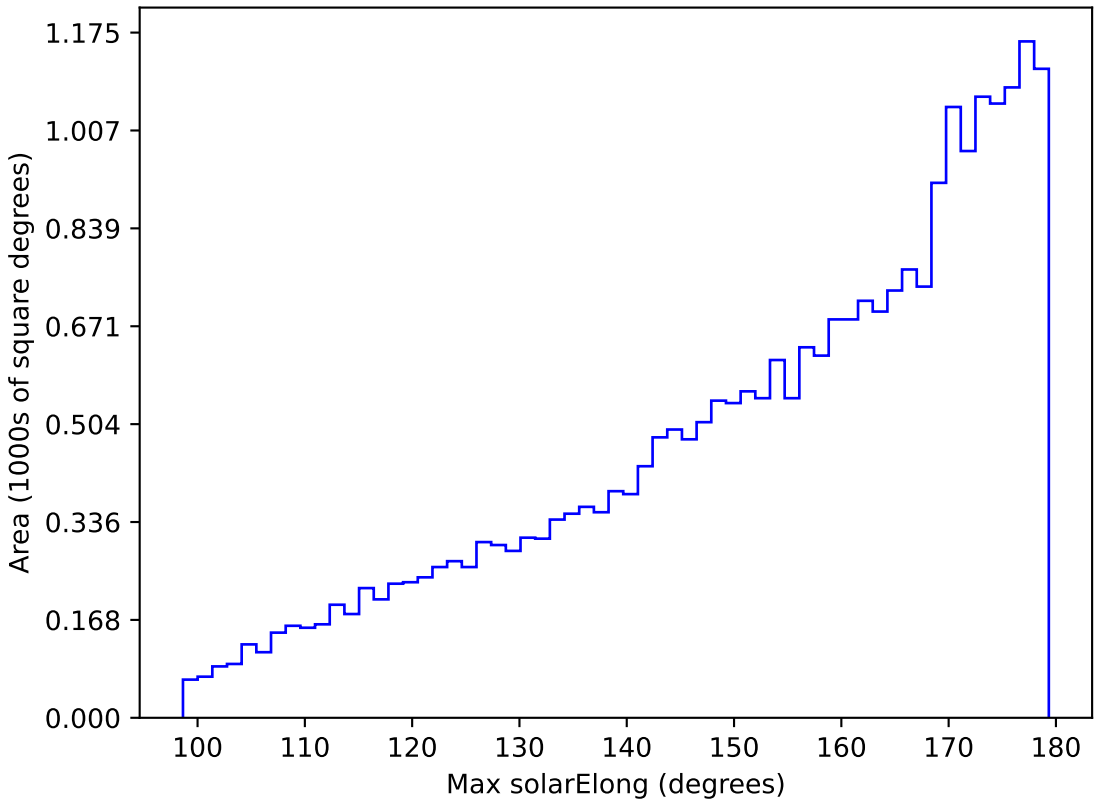
too_elab_r64_d2_giz_v3.4_10yrs All sky z band: Max solarElong
