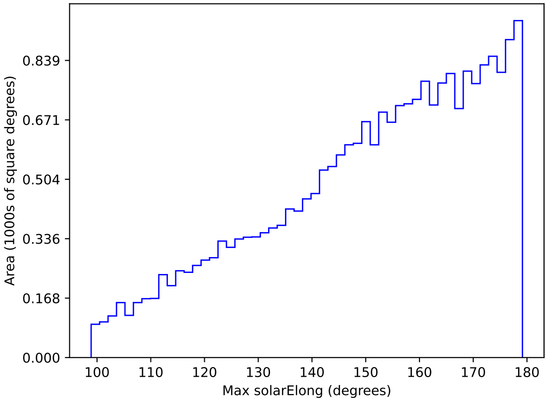
too_elab_r64_d2_giz_v3.4_10yrs All sky y band: Max solarElong
