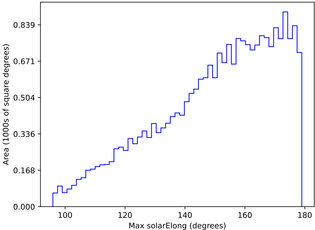
too_elab_r64_d2_giz_v3.4_10yrs All sky u band: Max solarElong
