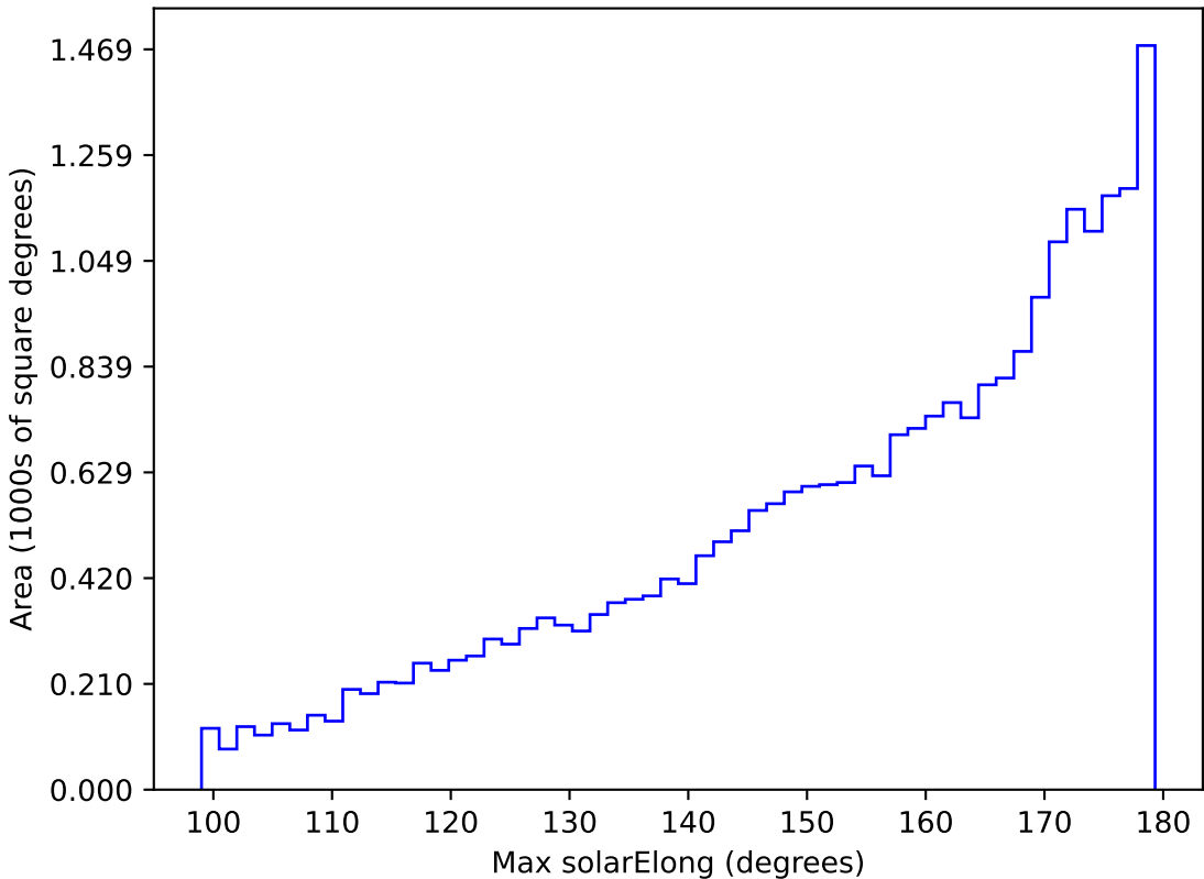
too_elab_r64_d2_giz_v3.4_10yrs All sky r band: Max solarElong
