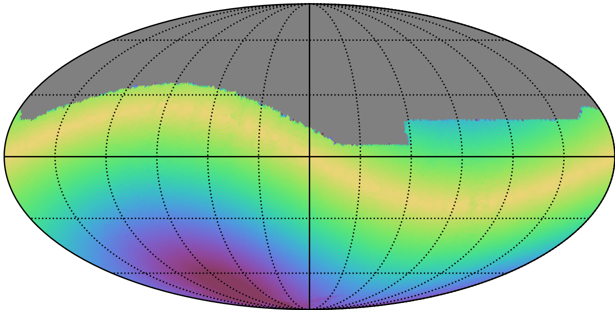
too_elab_r64_d2_giz_v3.4_10yrs All sky i band: Max solarElong
