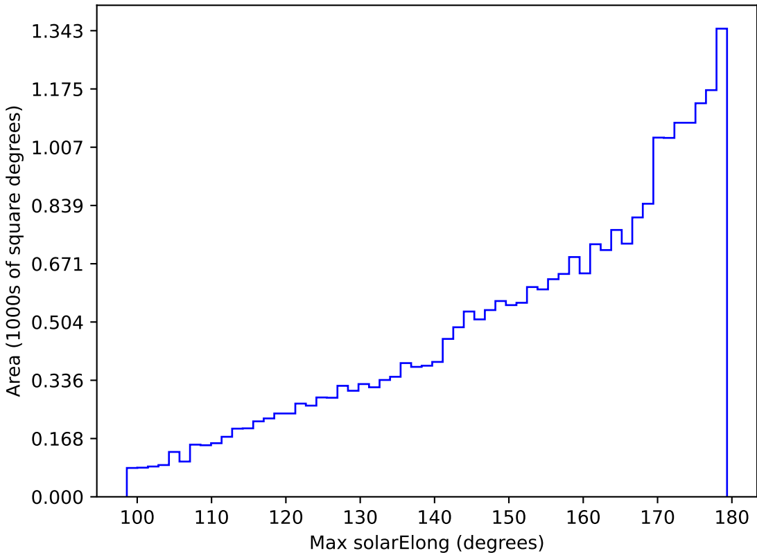
too_elab_r64_d2_giz_v3.4_10yrs All sky i band: Max solarElong
