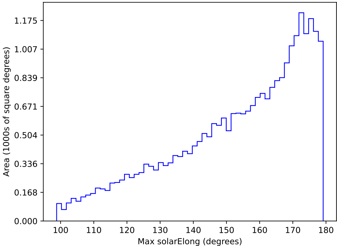
too_elab_r64_d2_giz_v3.4_10yrs All sky g band: Max solarElong
