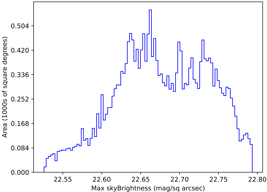
too_elab_r64_d2_giz_v3.4_10yrs Yr 1 u band: Max skyBrightness
