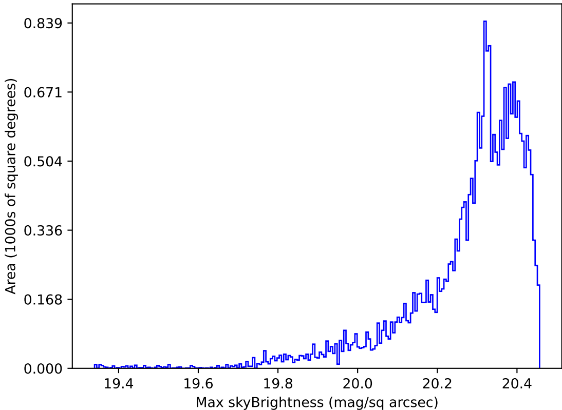
too_elab_r64_d2_giz_v3.4_10yrs Yr 1 i band: Max skyBrightness
