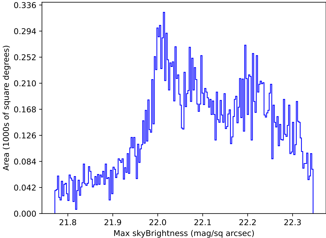
too_elab_r64_d2_giz_v3.4_10yrs Yr 1 g band: Max skyBrightness
