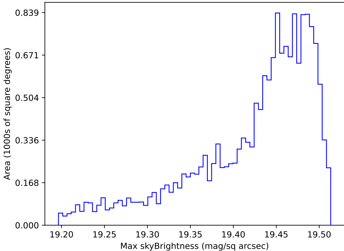
too_elab_r64_d2_giz_v3.4_10yrs WFD z band: Max skyBrightness
