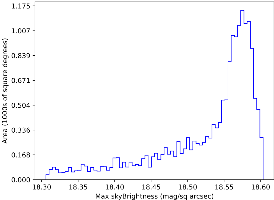
too_elab_r64_d2_giz_v3.4_10yrs WFD y band: Max skyBrightness
