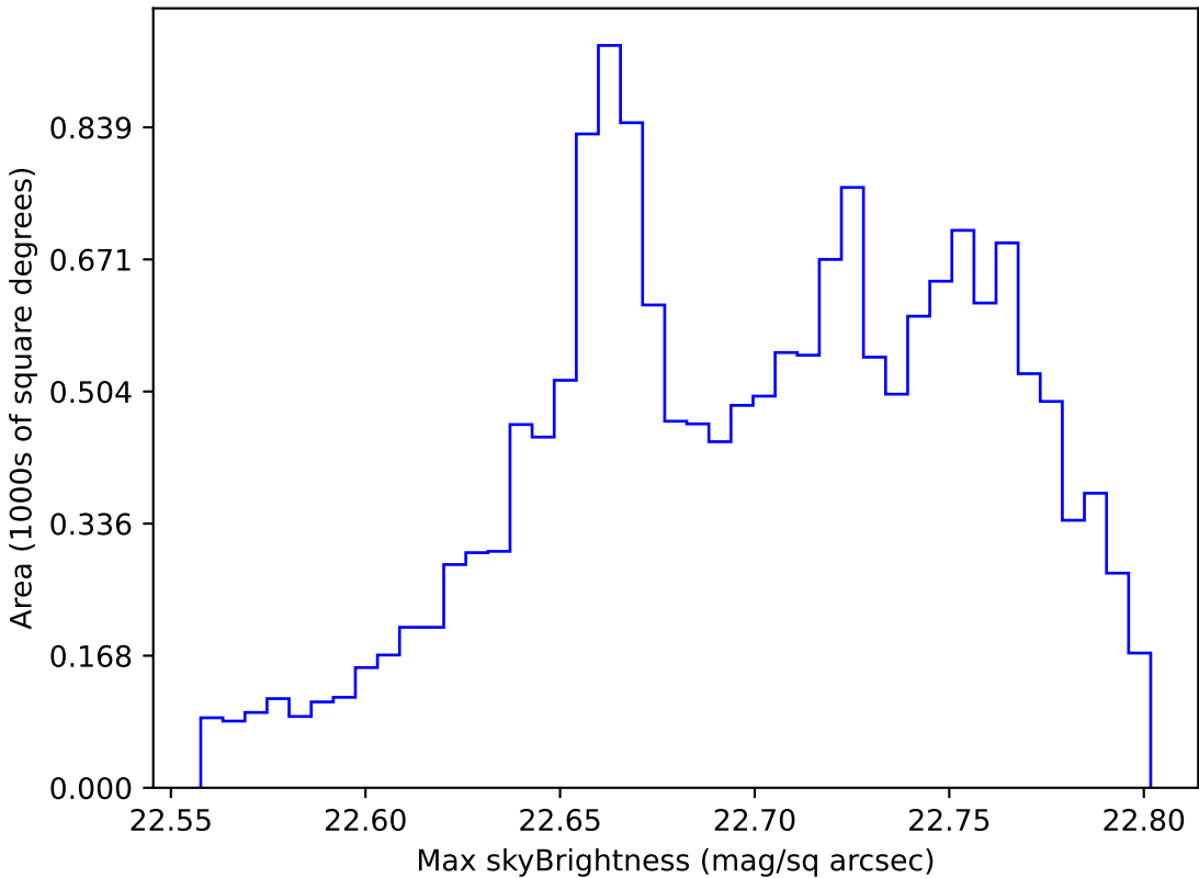
too_elab_r64_d2_giz_v3.4_10yrs WFD u band: Max skyBrightness
