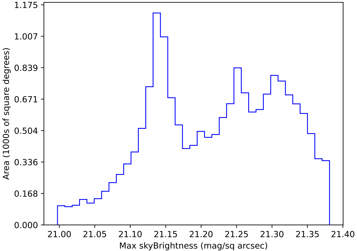
too_elab_r64_d2_giz_v3.4_10yrs WFD r band: Max skyBrightness
