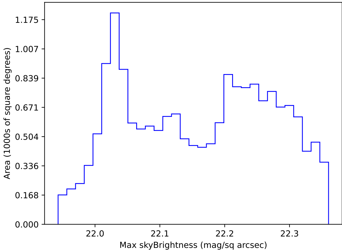
too_elab_r64_d2_giz_v3.4_10yrs WFD g band: Max skyBrightness
