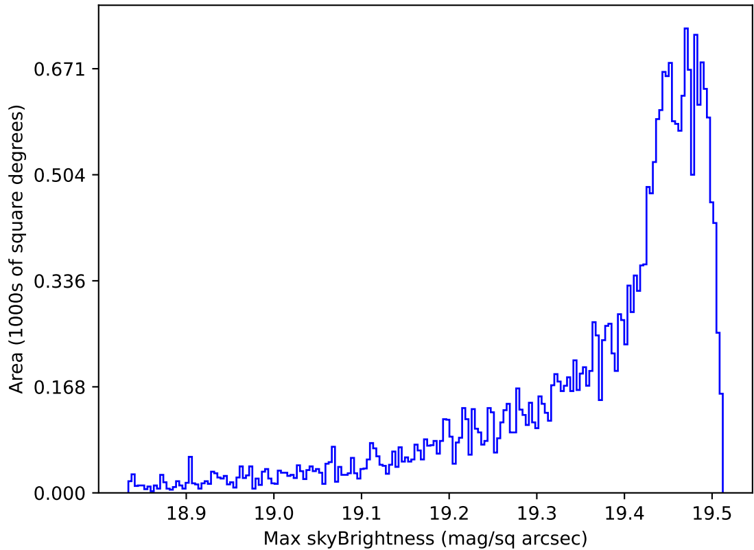
too_elab_r64_d2_giz_v3.4_10yrs All sky z band: Max skyBrightness
