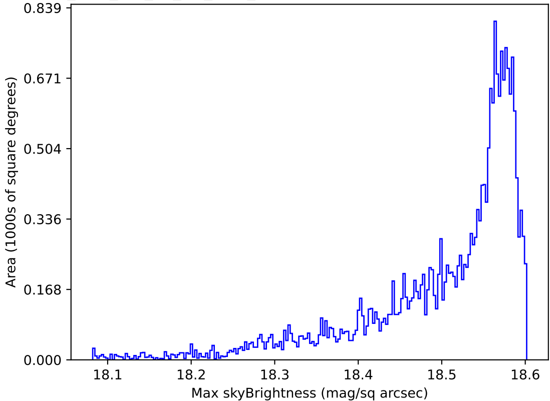
too_elab_r64_d2_giz_v3.4_10yrs All sky y band: Max skyBrightness
