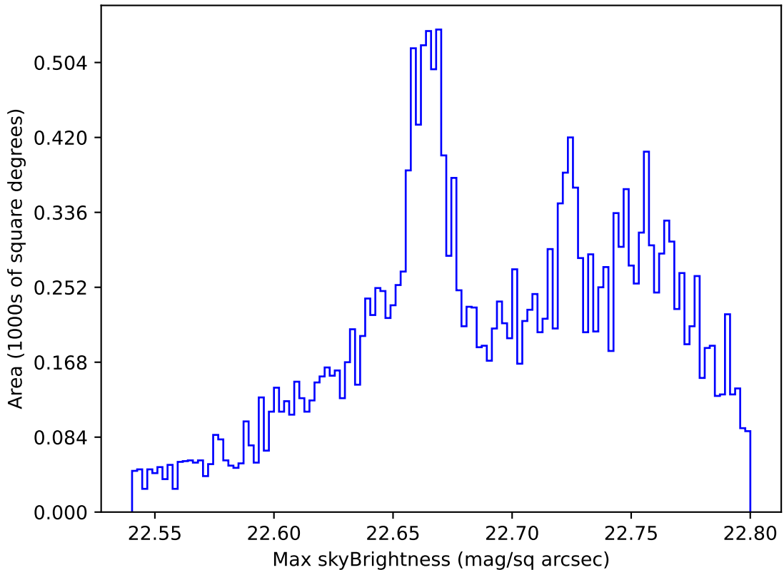
too_elab_r64_d2_giz_v3.4_10yrs All sky u band: Max skyBrightness
