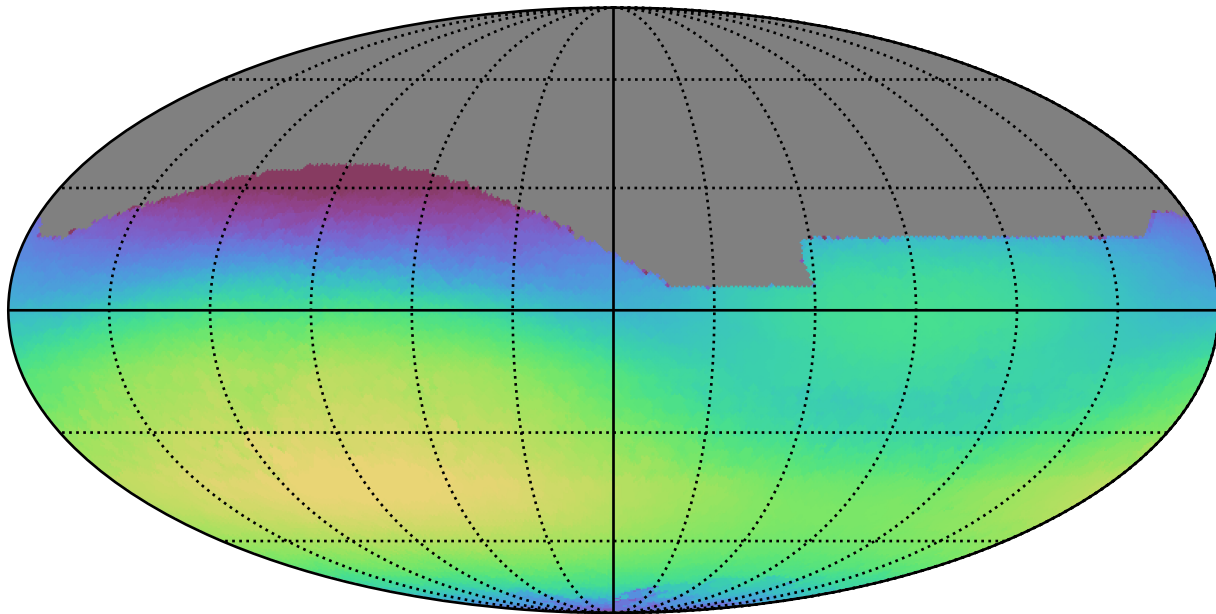
too_elab_r64_d2_giz_v3.4_10yrs All sky r band: Max skyBrightness
