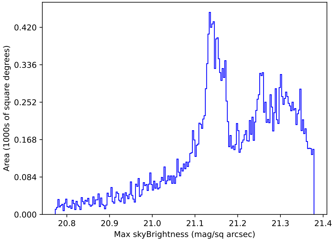
too_elab_r64_d2_giz_v3.4_10yrs All sky r band: Max skyBrightness
