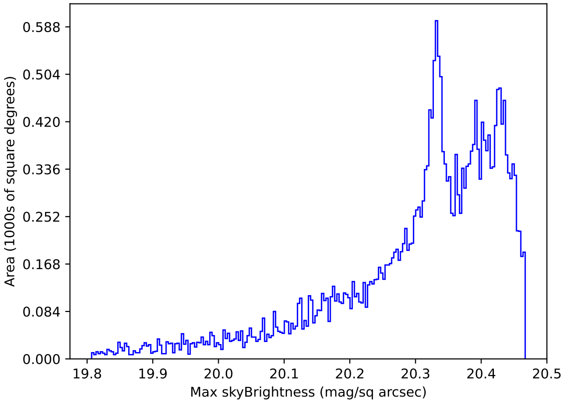
too_elab_r64_d2_giz_v3.4_10yrs All sky i band: Max skyBrightness
