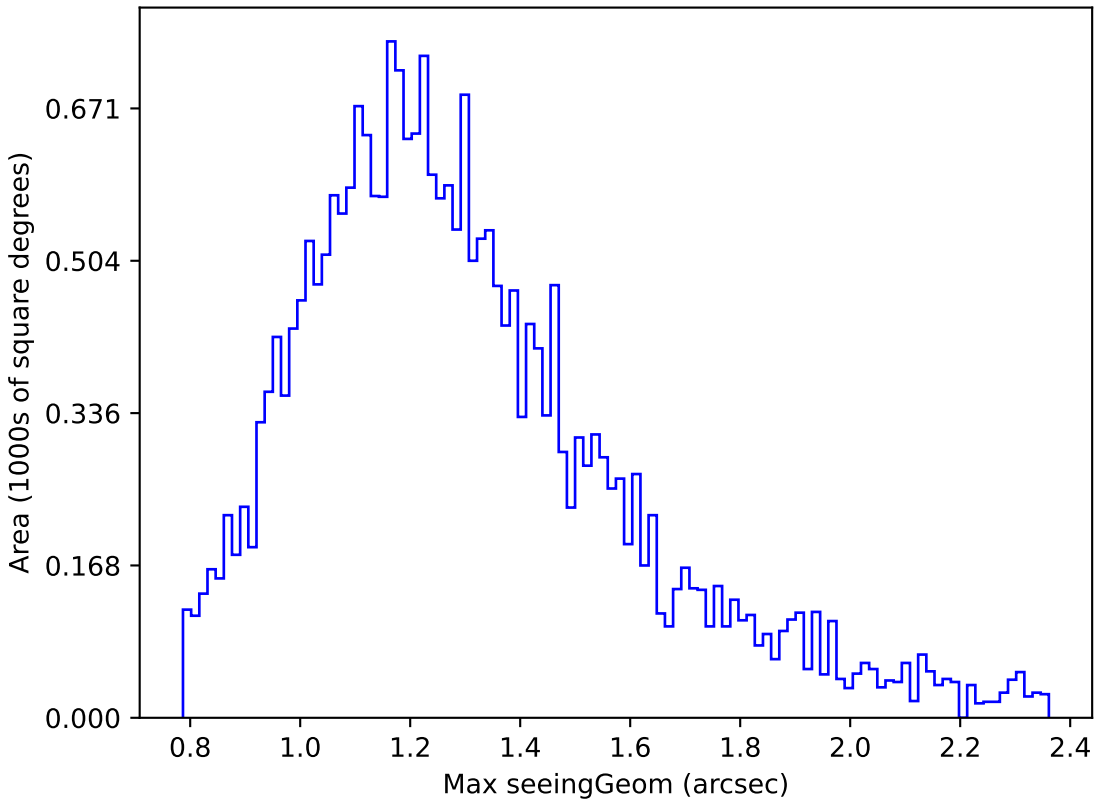
too_elab_r64_d2_giz_v3.4_10yrs Yr 1 z band: Max seeingGeom
