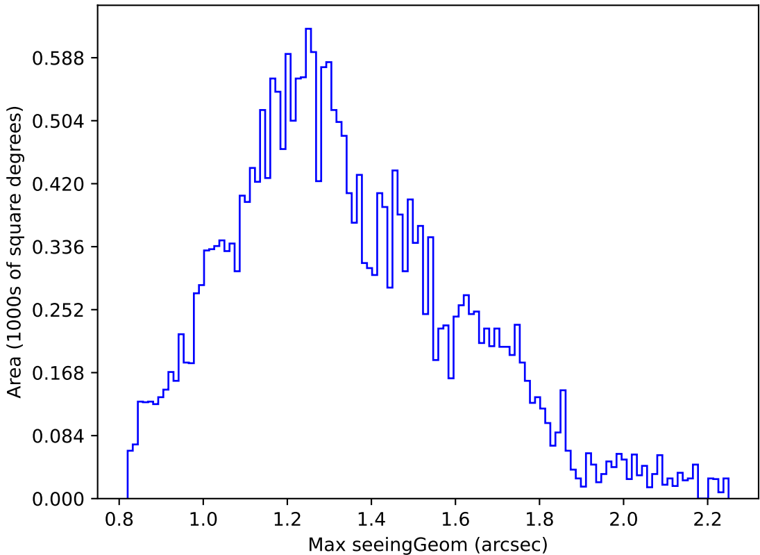
too_elab_r64_d2_giz_v3.4_10yrs Yr 1 r band: Max seeingGeom
