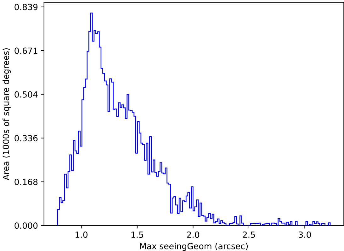
too_elab_r64_d2_giz_v3.4_10yrs Yr 1 g band: Max seeingGeom
