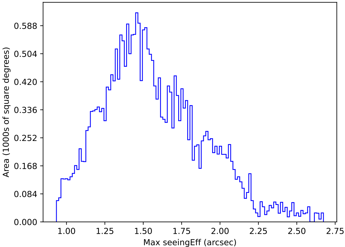
too_elab_r64_d2_giz_v3.4_10yrs Yr 1 r band: Max seeingEff
