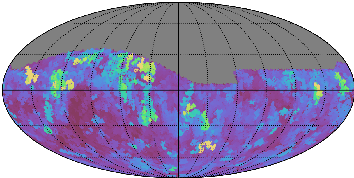
too_elab_r64_d2_giz_v3.4_10yrs Yr 1 i band: Max seeingEff
