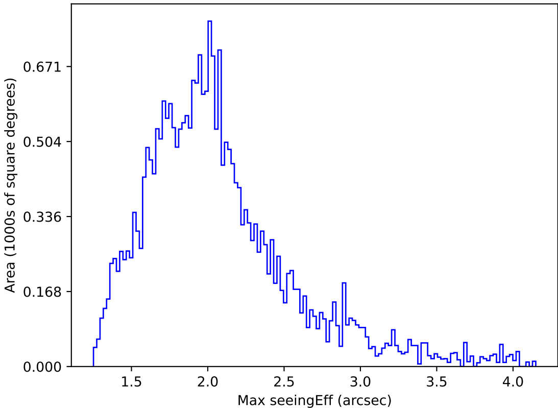
too_elab_r64_d2_giz_v3.4_10yrs Yr 1 all bands: Max seeingEff
