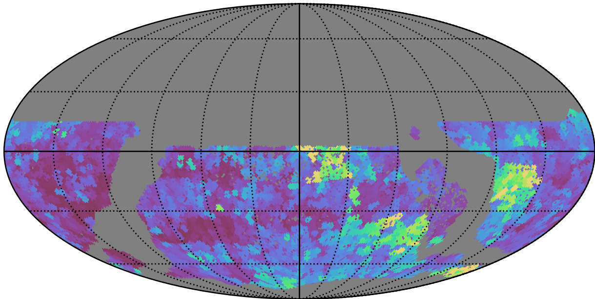
too_elab_r64_d2_giz_v3.4_10yrs WFD y band: Max seeingEff
