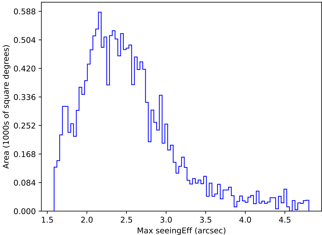
too_elab_r64_d2_giz_v3.4_10yrs WFD y band: Max seeingEff
