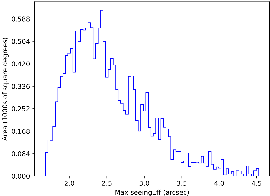
too_elab_r64_d2_giz_v3.4_10yrs WFD g band: Max seeingEff
