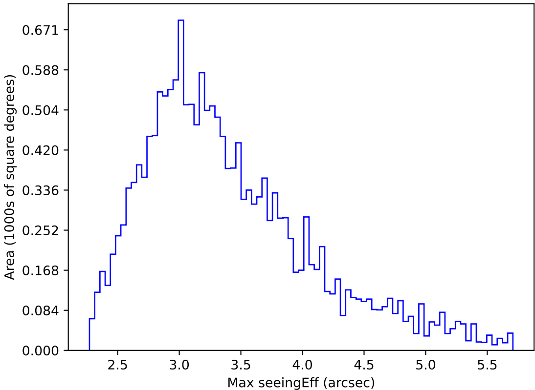
too_elab_r64_d2_giz_v3.4_10yrs WFD all bands: Max seeingEff
