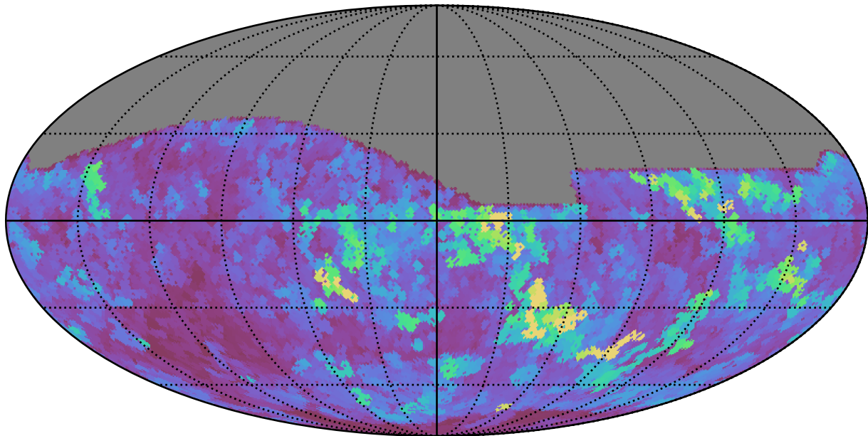
too_elab_r64_d2_giz_v3.4_10yrs All sky z band: Max seeingEff
