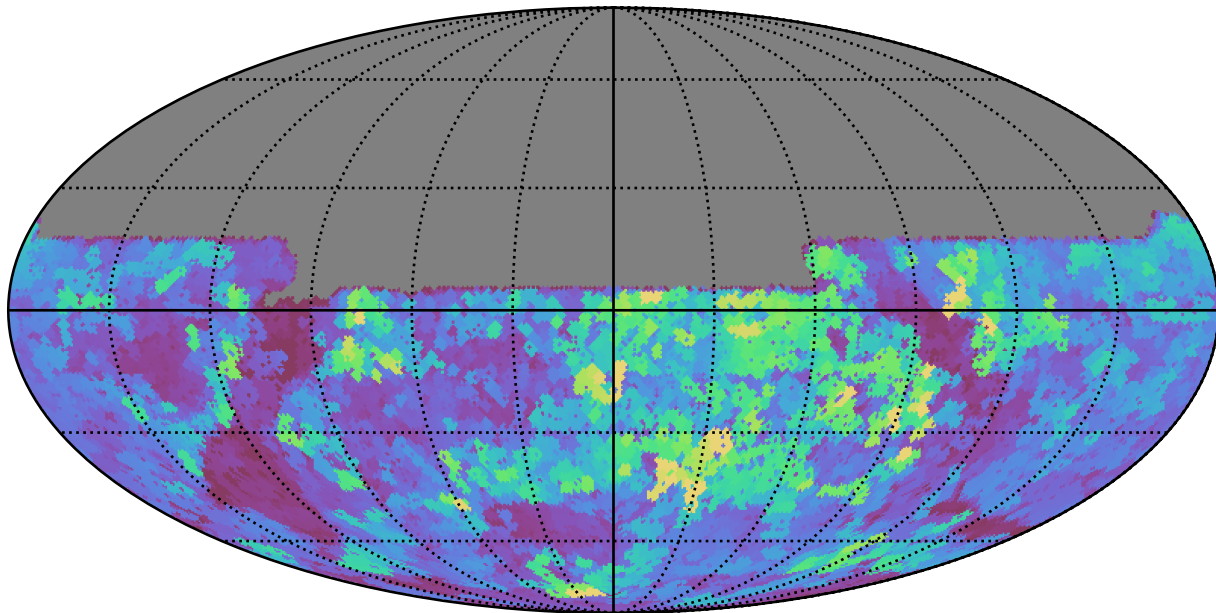
too_elab_r64_d2_giz_v3.4_10yrs All sky u band: Max seeingEff
