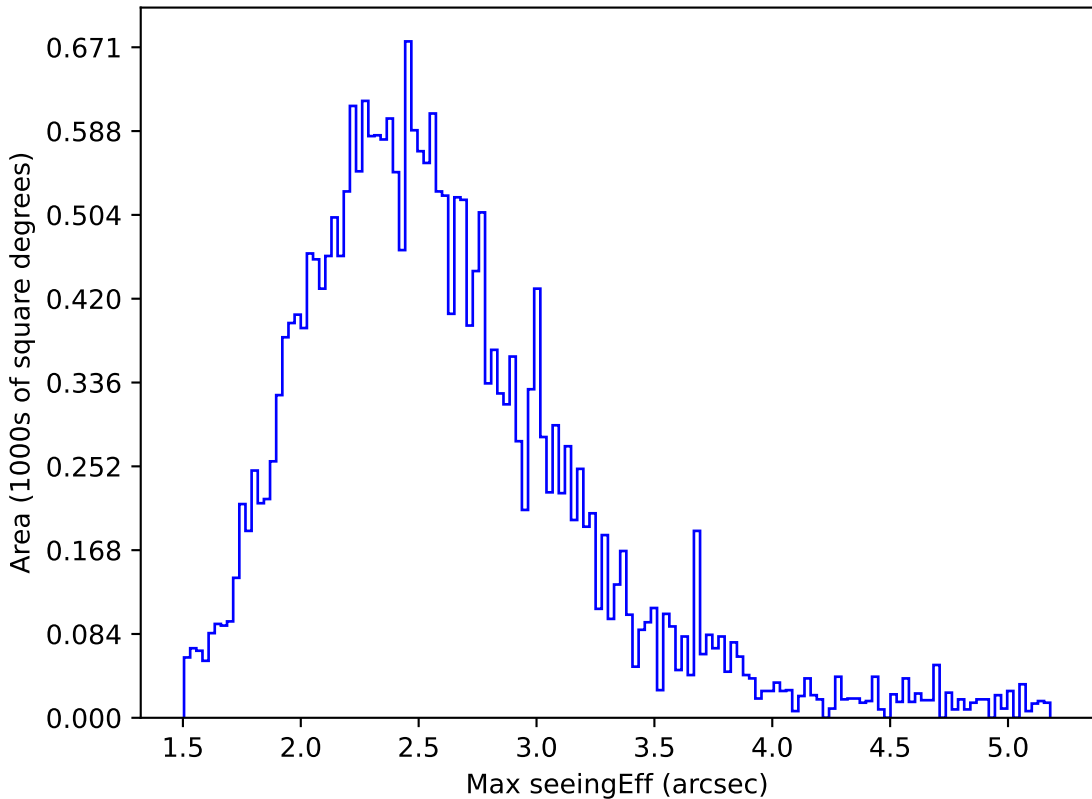
too_elab_r64_d2_giz_v3.4_10yrs All sky i band: Max seeingEff
