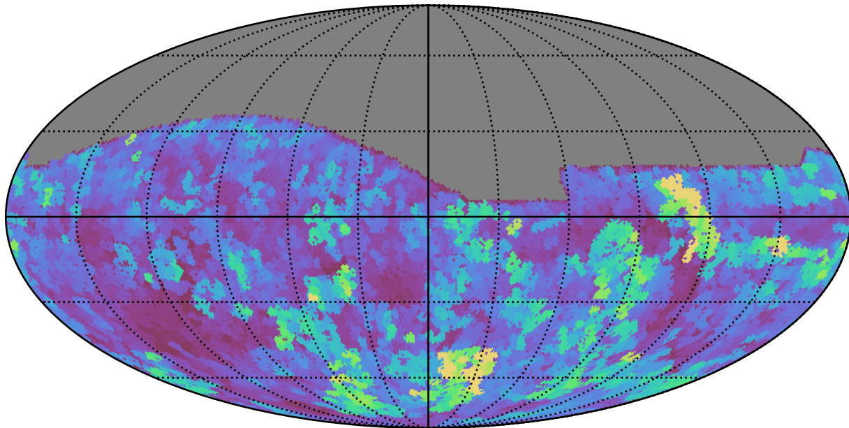
too_elab_r64_d2_giz_v3.4_10yrs All sky g band: Max seeingEff
