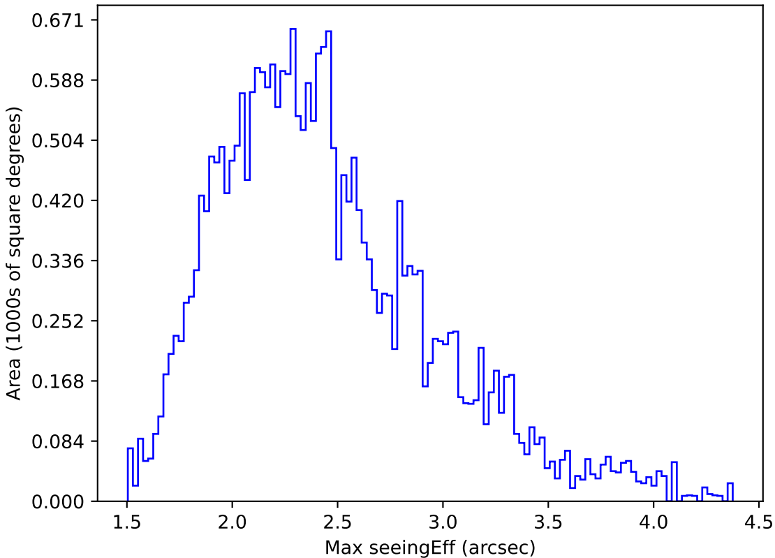
too_elab_r64_d2_giz_v3.4_10yrs All sky g band: Max seeingEff
