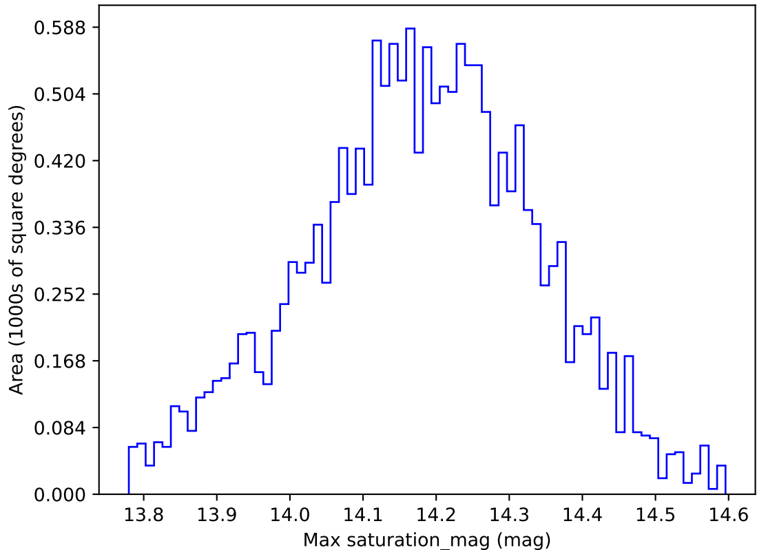
too_elab_r64_d2_giz_v3.4_10yrs WFD y band: Max saturation_mag
