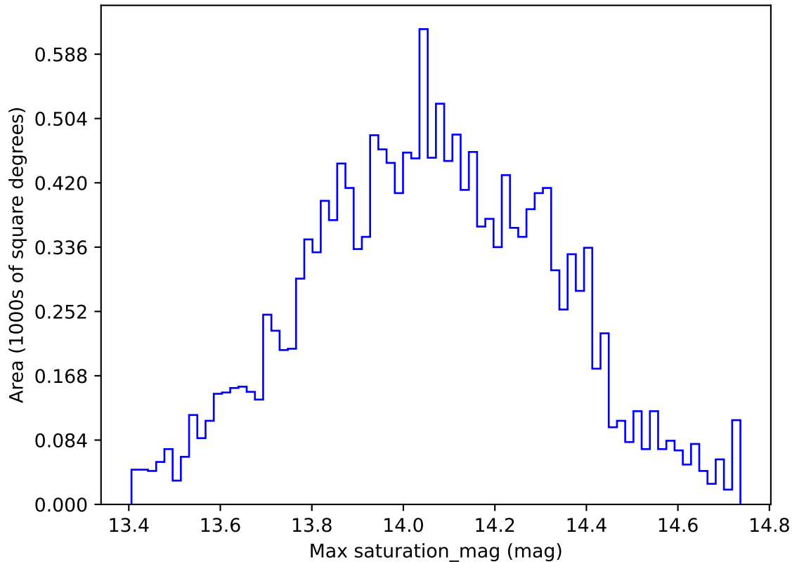
too_elab_r64_d2_giz_v3.4_10yrs WFD u band: Max saturation_mag
