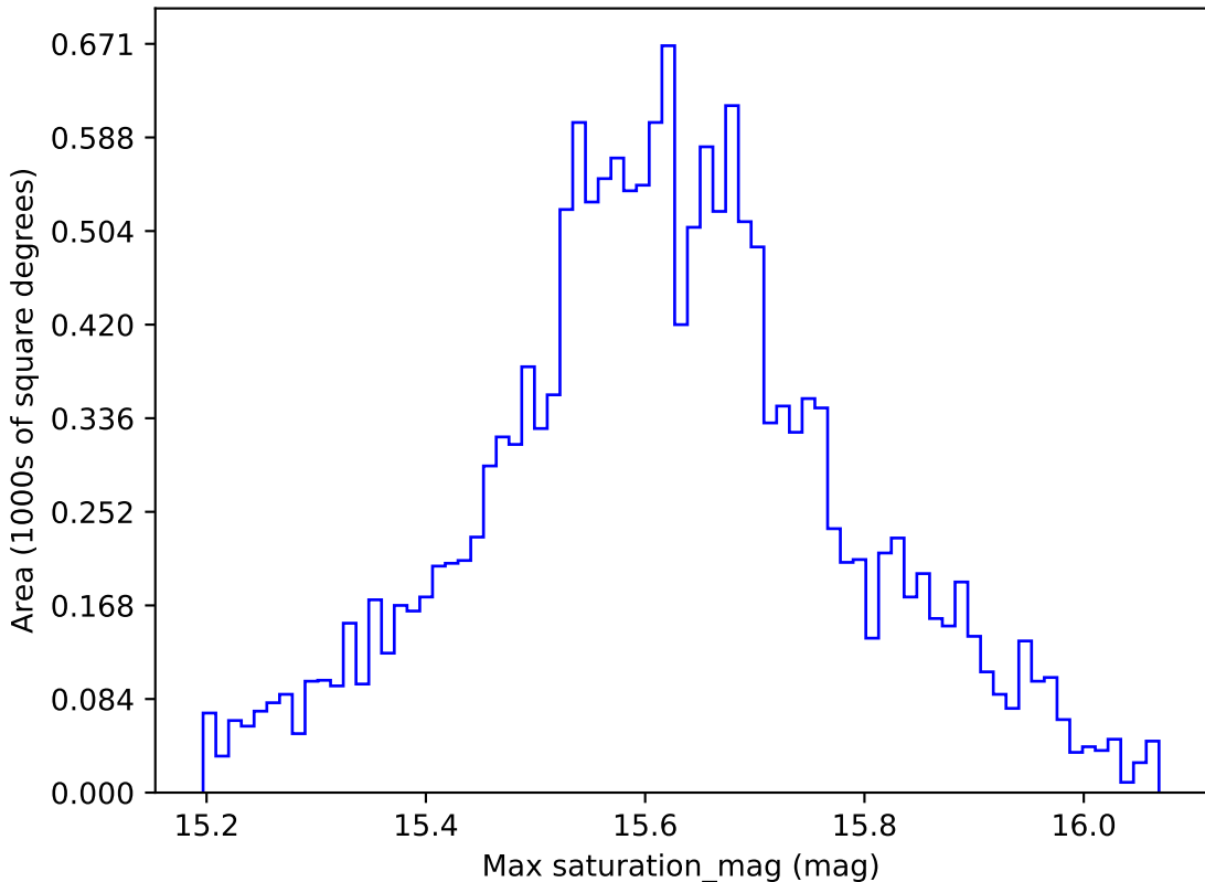
too_elab_r64_d2_giz_v3.4_10yrs WFD i band: Max saturation_mag
