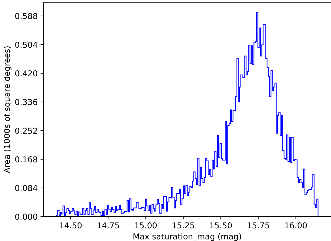
too_elab_r64_d2_giz_v3.4_10yrs All sky r band: Max saturation_mag
