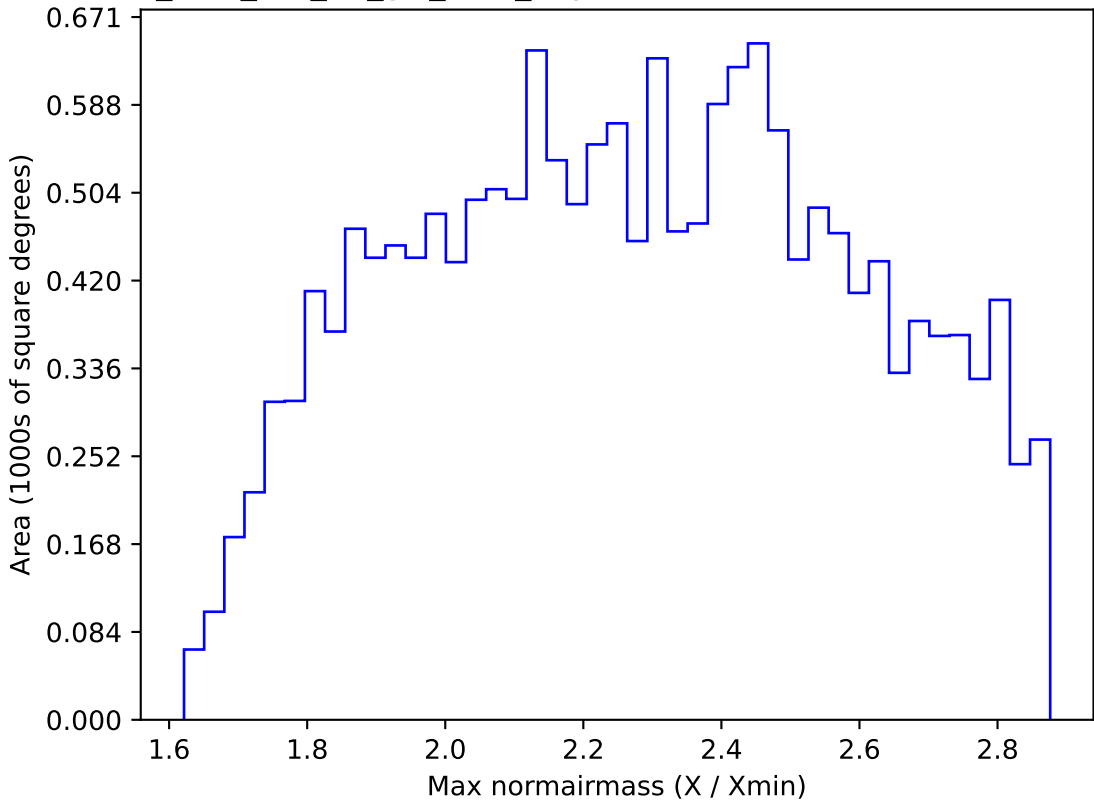
too_elab_r64_d2_giz_v3.4_10yrs WFD z band: Max normairmass
